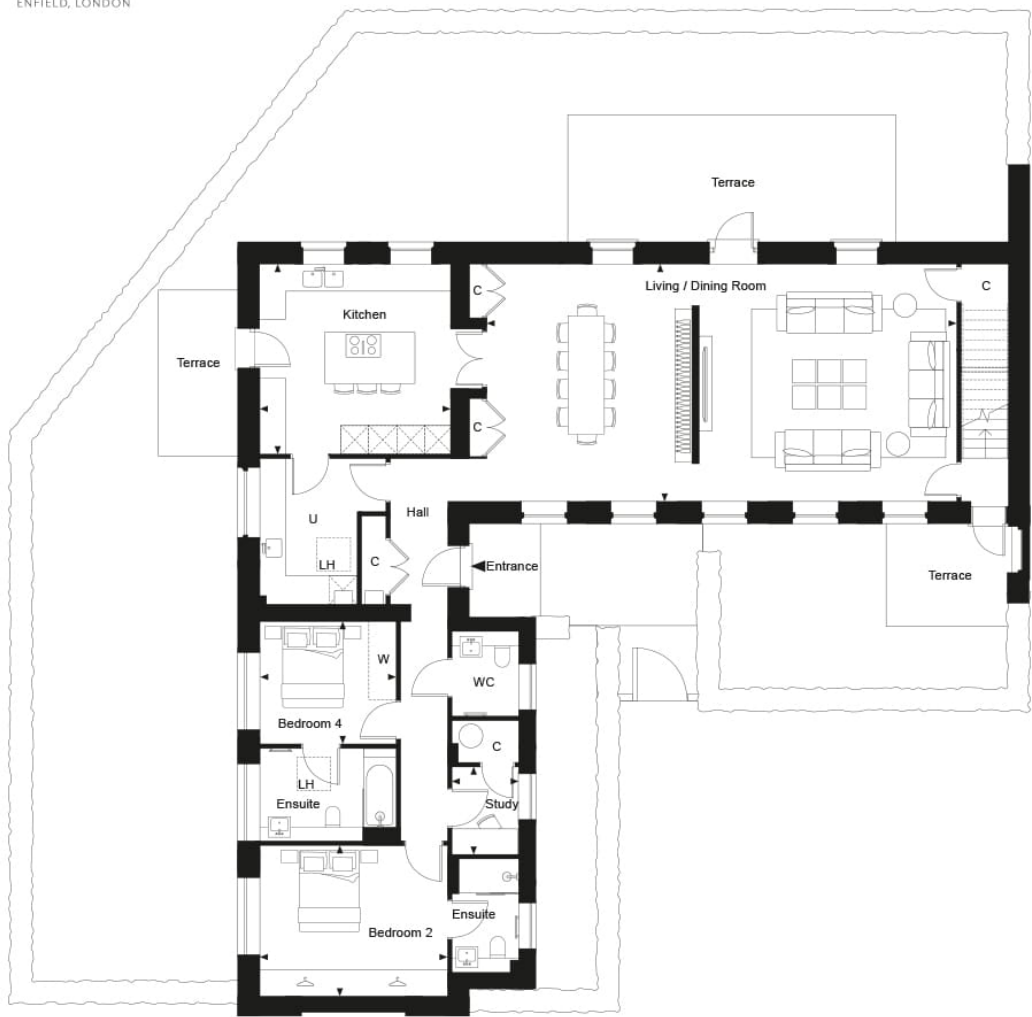
Trent Park, The Stable Block - Property 01, Ground Floor
